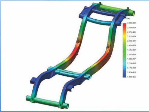
Product Design- Analysis/simulation
